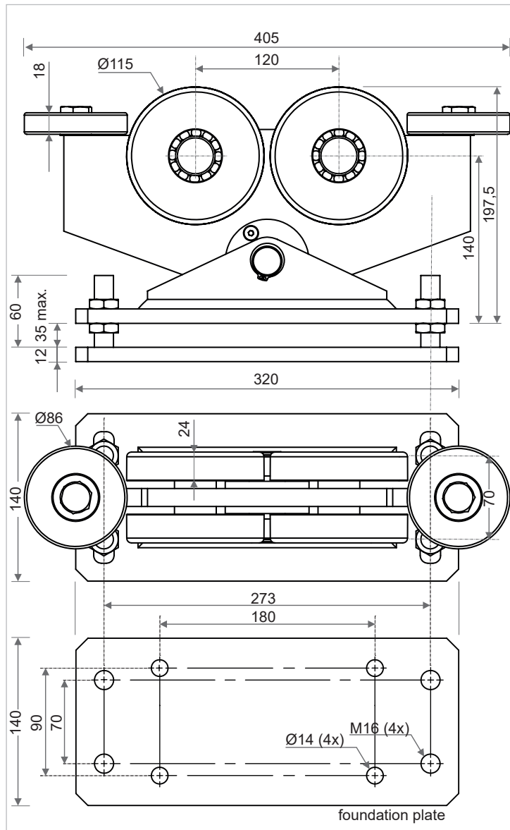
Guide-in bracket Rollco® LWS 125
