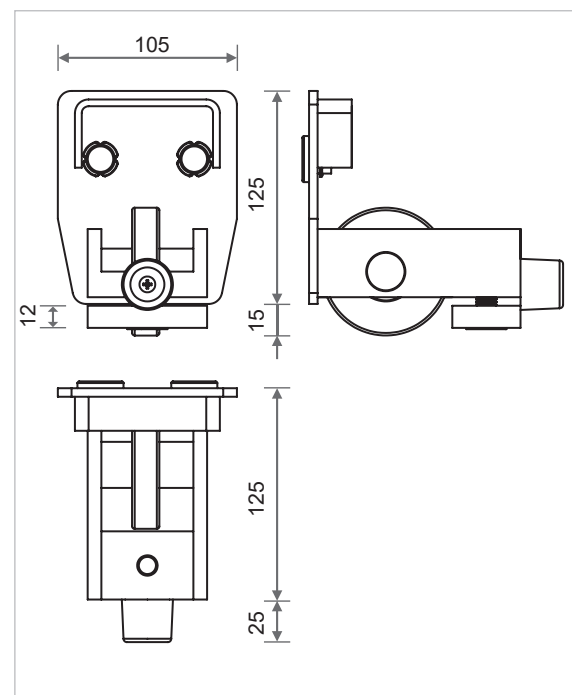
End plate with roller Rollco® LWS 125
