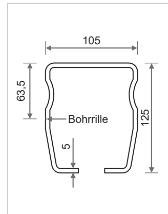
Track Rollco® LWS 125
