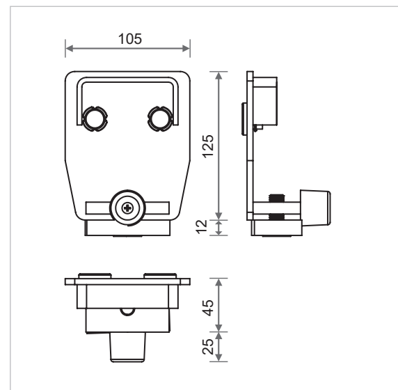
End plates Rollco® LWS 125
