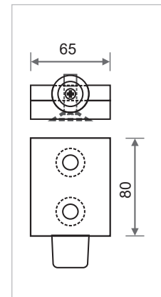
End stops Rollco® LWS 125
