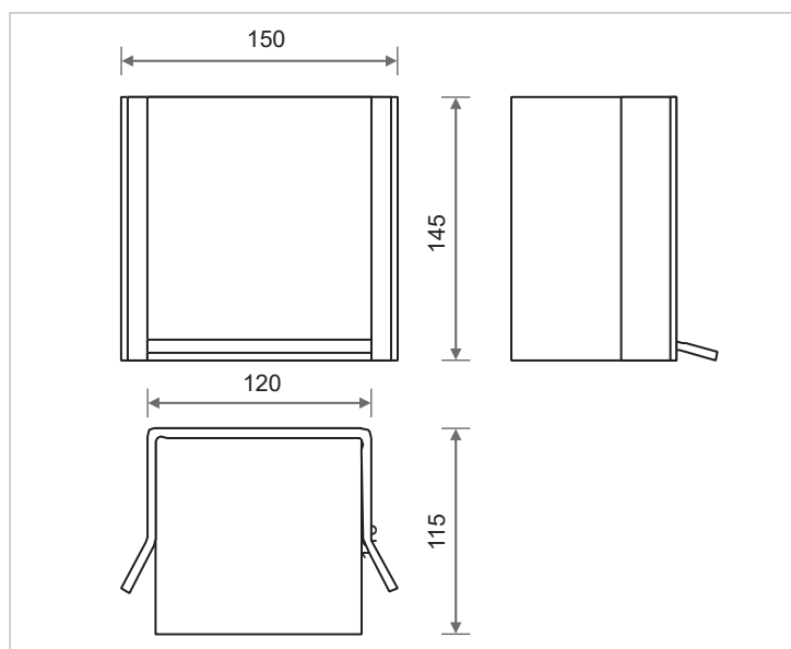
Guide-in bracket Rollco® LWS 125
